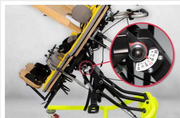
Angle scale
