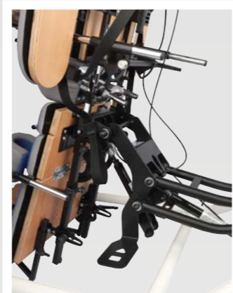
Recline adjustment
