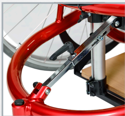
Tilt adjustment
